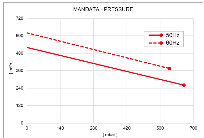
Curve riferite alla pressione di 1013mbar (Ass.) e temperatura 20°C (tolleranza \pm 10%) Curves refer to 1013mbar (Abs.) pressure and 20°C temperature (tolerance \pm 10%)
