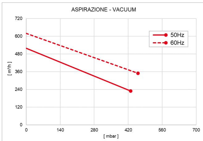
Curve riferite alla pressione di 1013mbar (Ass.) e temperatura 20°C (tolleranza \pm 10%) Curves refer to 1013mbar (Abs.) pressure and 20°C temperature (tolerance \pm 10%)
